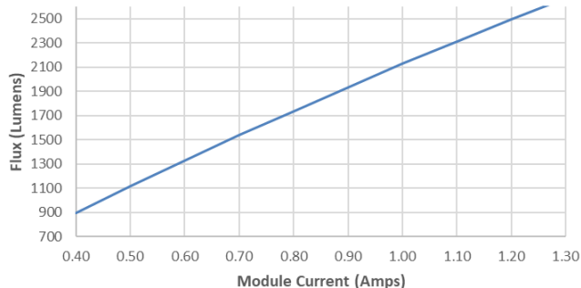
Flux vs Current - M10CC840D32N3W
