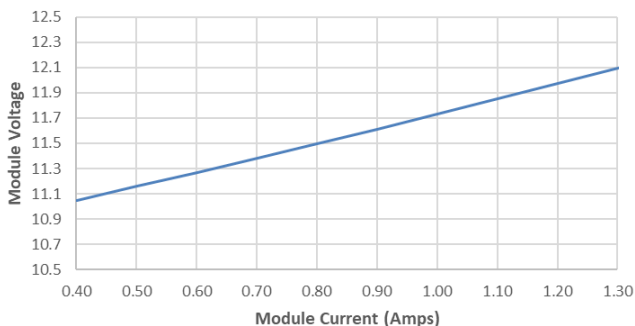
Voltage vs Current - M10CC840D32N3W
