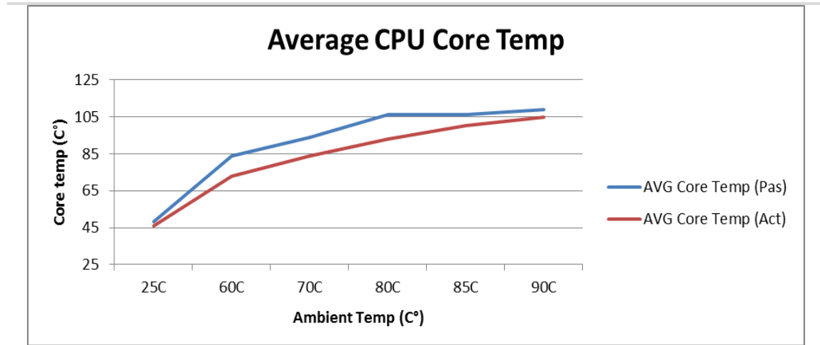
Figure 32. EBX-38ECP CPU Core Temperature Relative to Ambient Temperature
