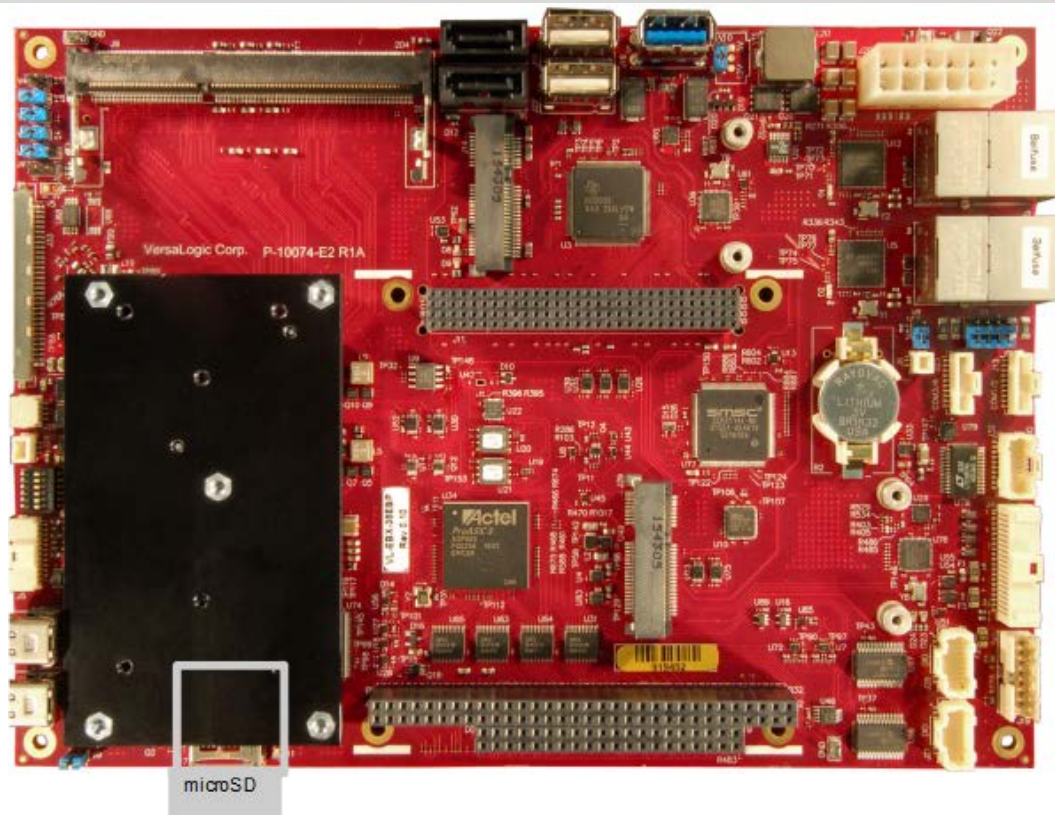
Figure 12. Location of the microSD Socket
