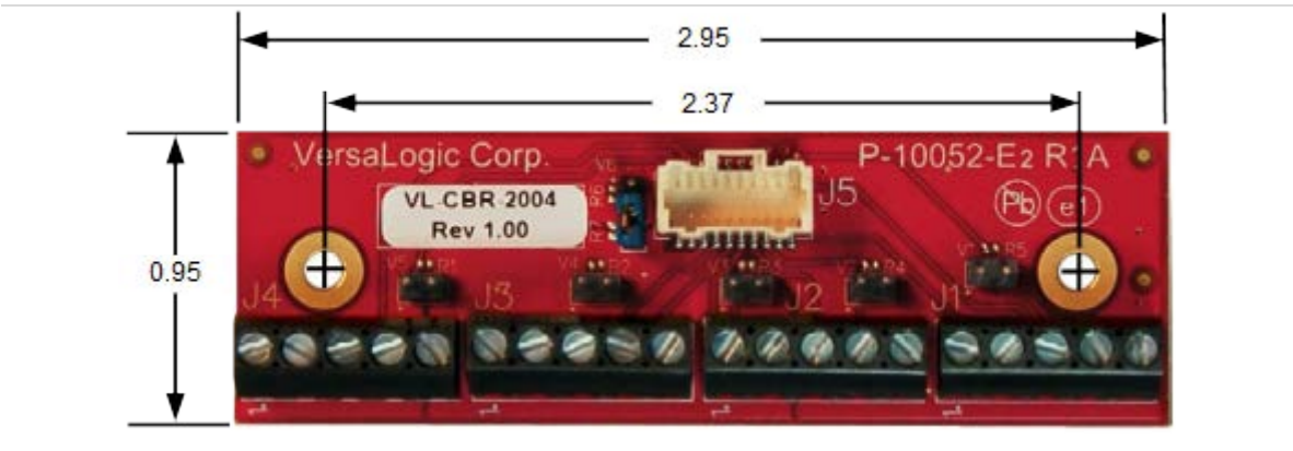
Figure 29. CBR-2004 Dimensions
