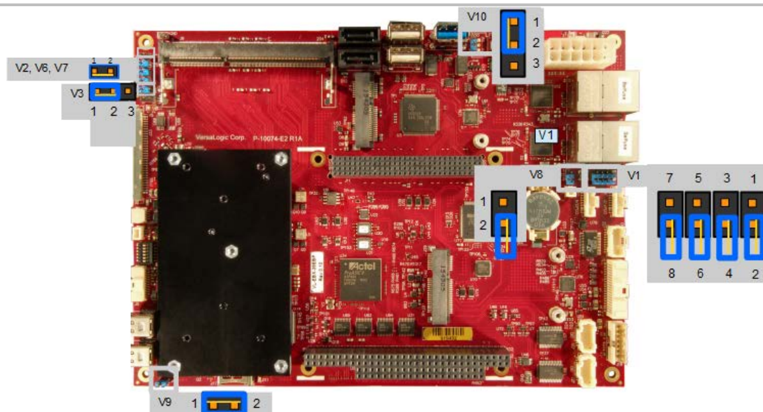
Figure 5. Jumpers Blocks in the As-Shipped Configuration
