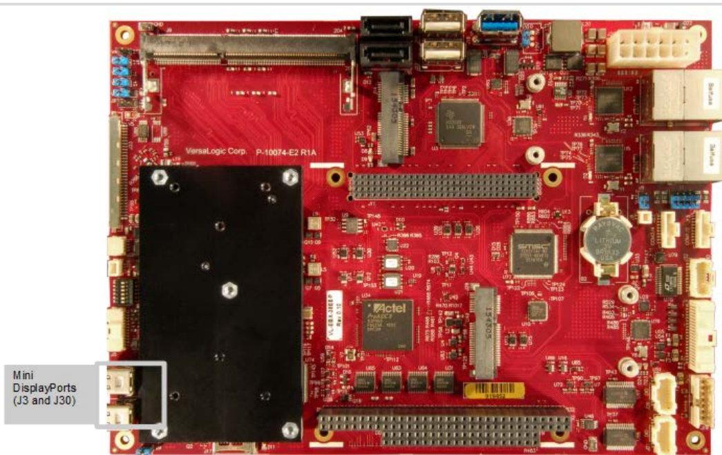
Figure 20. Location of the Mini DisplayPort Connectors
