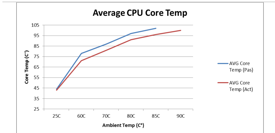
Figure 30. EBX-38EAP CPU Core Temperature Relative to Ambient Temperature
