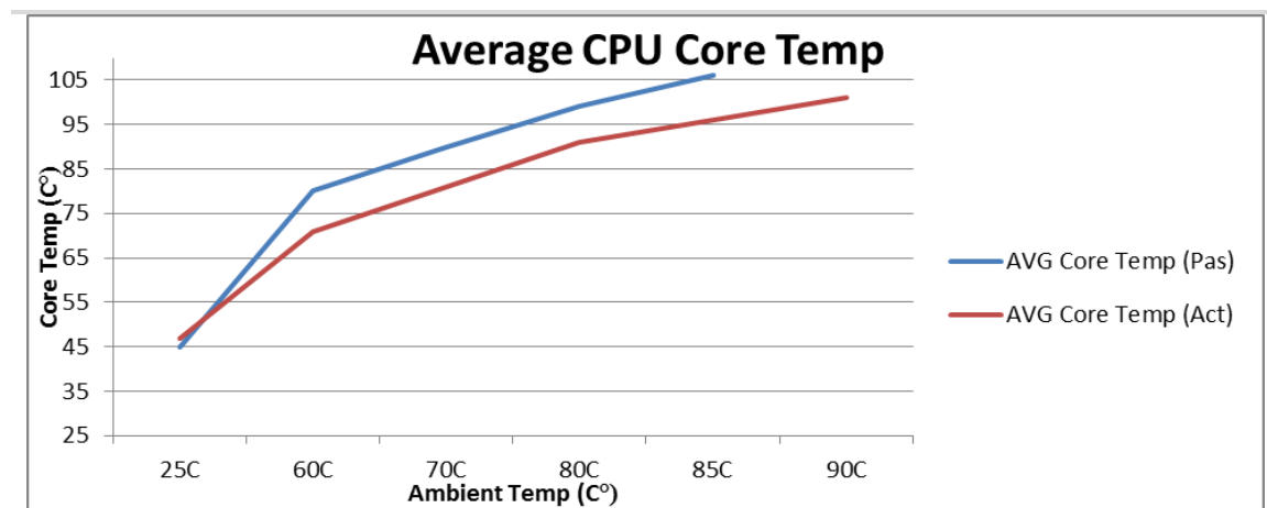
Figure 31. EBX-38EBP CPU Core Temperature Relative to Ambient Temperature
