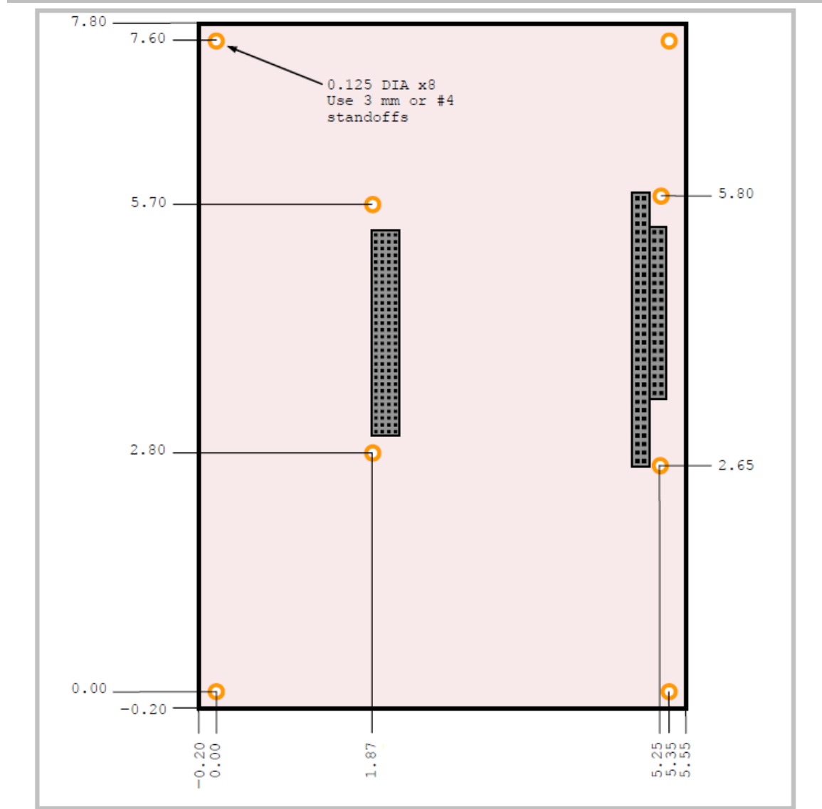
Figure 4. EBX-38 Dimensions and Mounting Holes
