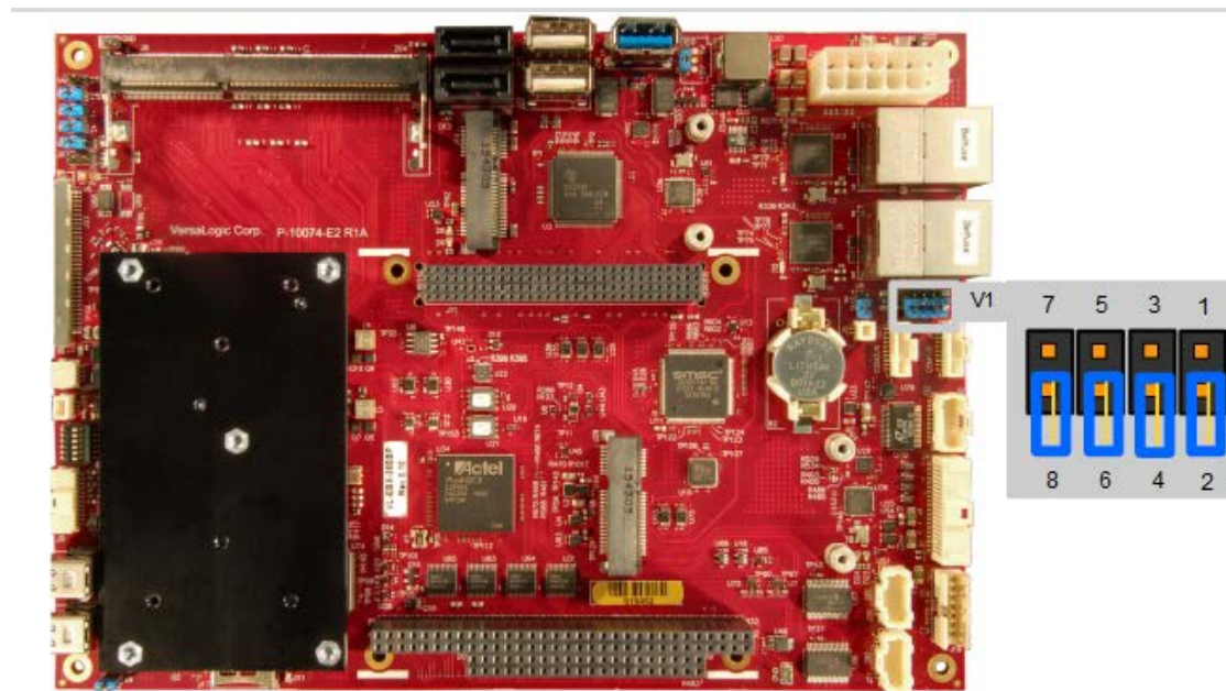
Figure 18. COM1/COM2/COM3/COM4 End-point Termination Jumpers
