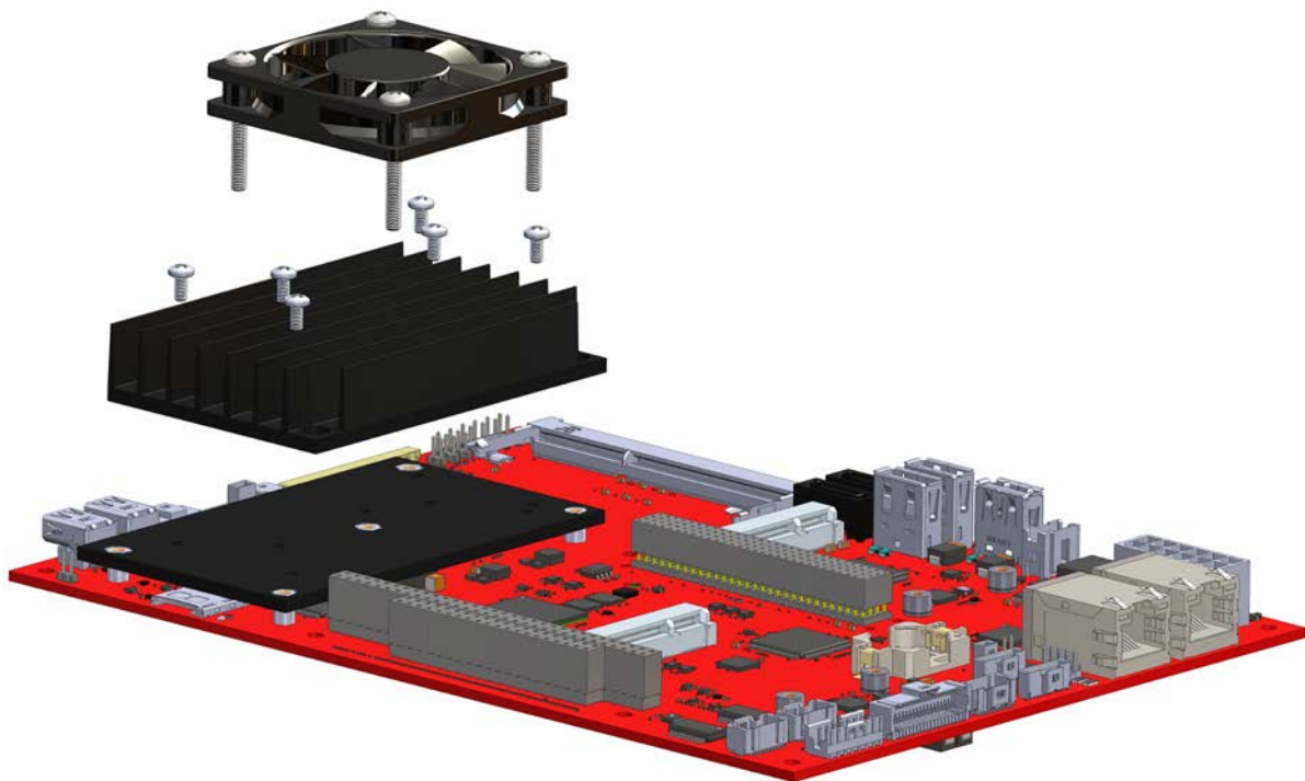
Figure 34. Installing the Heat Sink Fan
