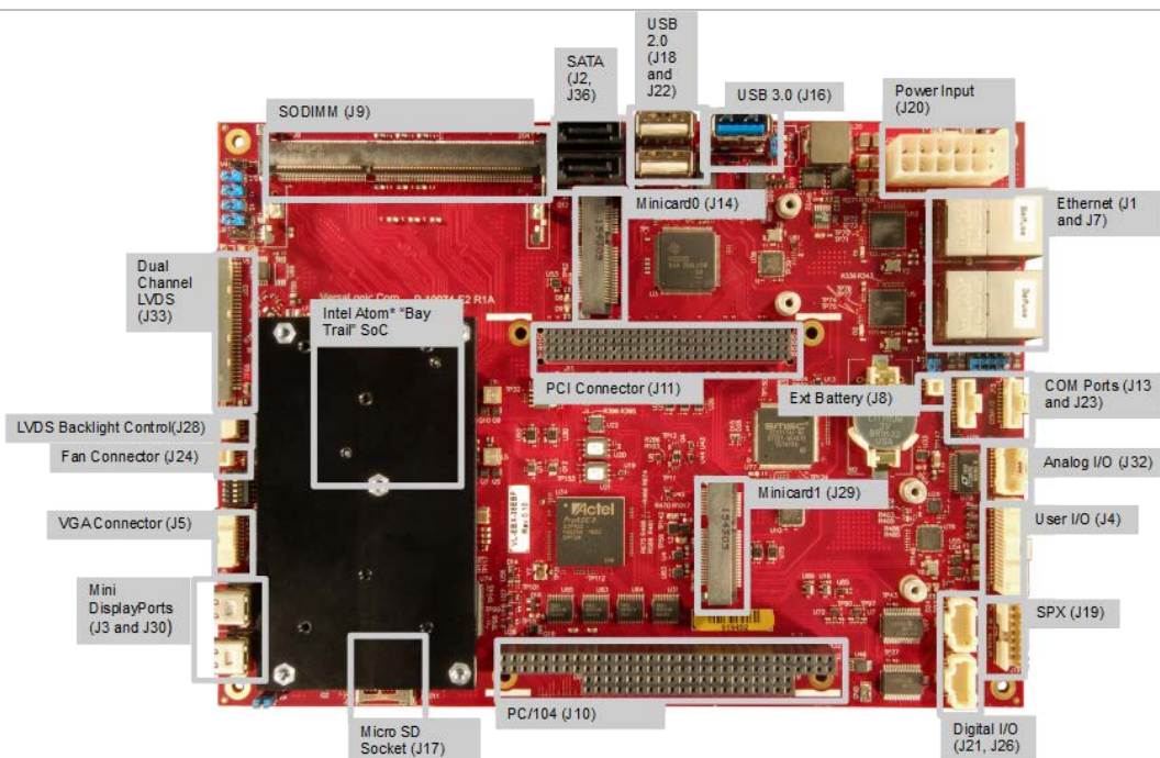
Figure 2. VL-EBX-38 Viper Single Board Computer (Top Side)
