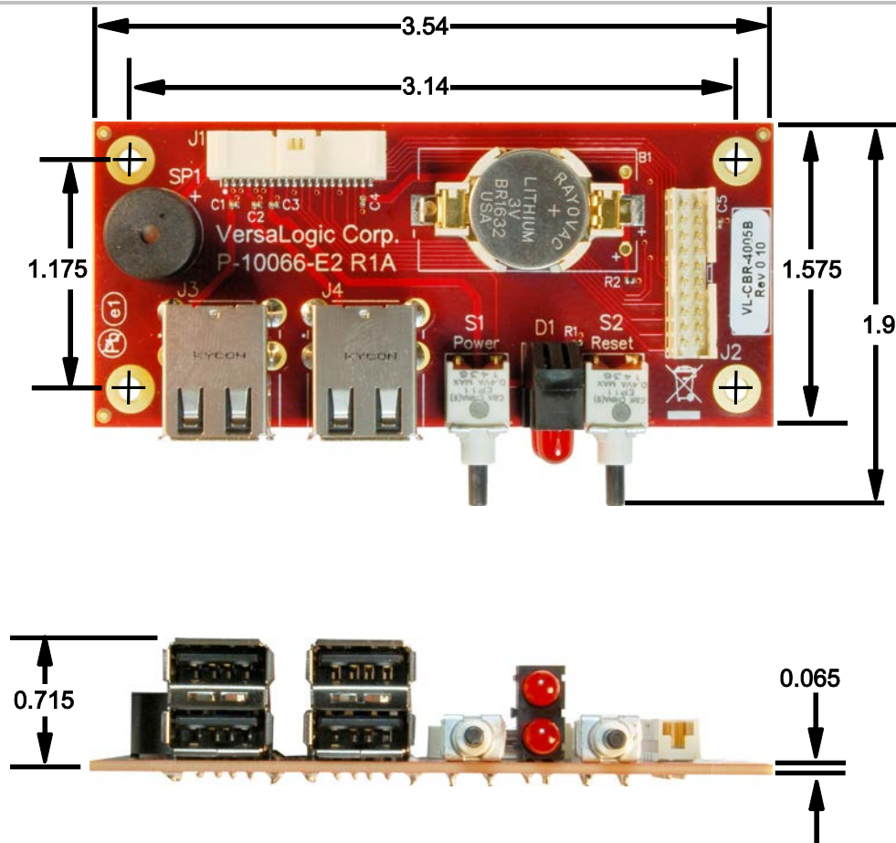
Figure 27. CBR-4005B Dimensions and Mounting Holes
