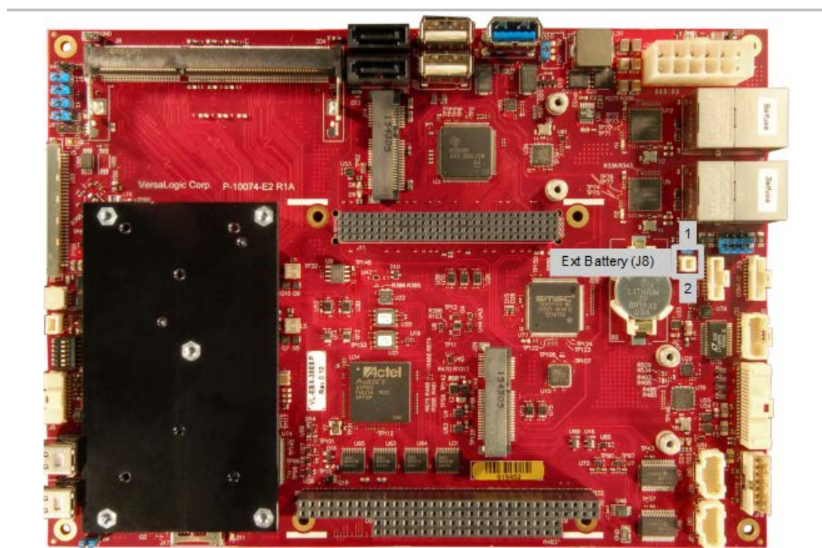
Figure 8. Location and Pin Orientation of the External Battery Connector
