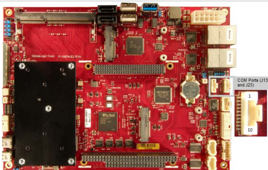
Figure 17. Location and Pin Orientation of Serial Port Connectors
