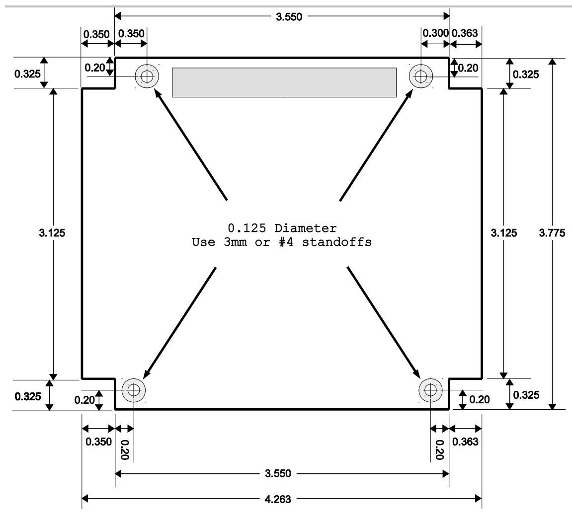
Figure 4. EPM-39 Dimensions and Mounting Holes
