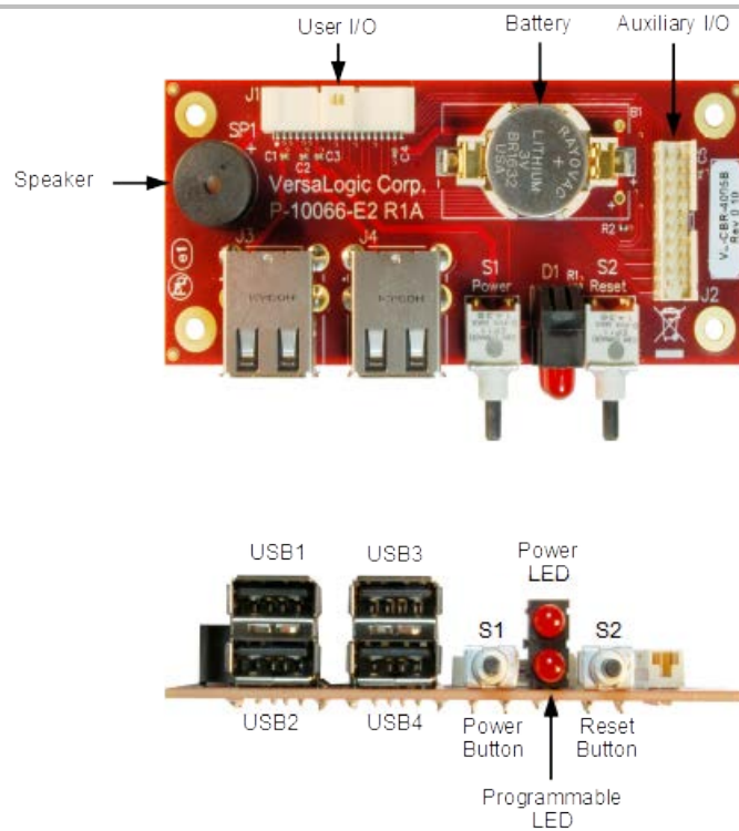
Figure 21. CBR-4005B Connectors, Switches, and LEDs
