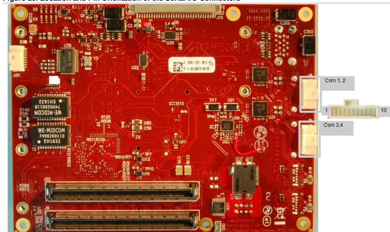
Figure 19. Location and Pin Orientation of the Serial I/O Connectors
