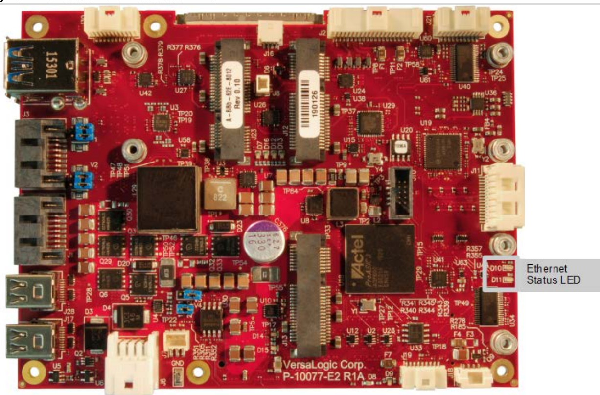
Figure 24. Onboard Ethernet Status LEDs
