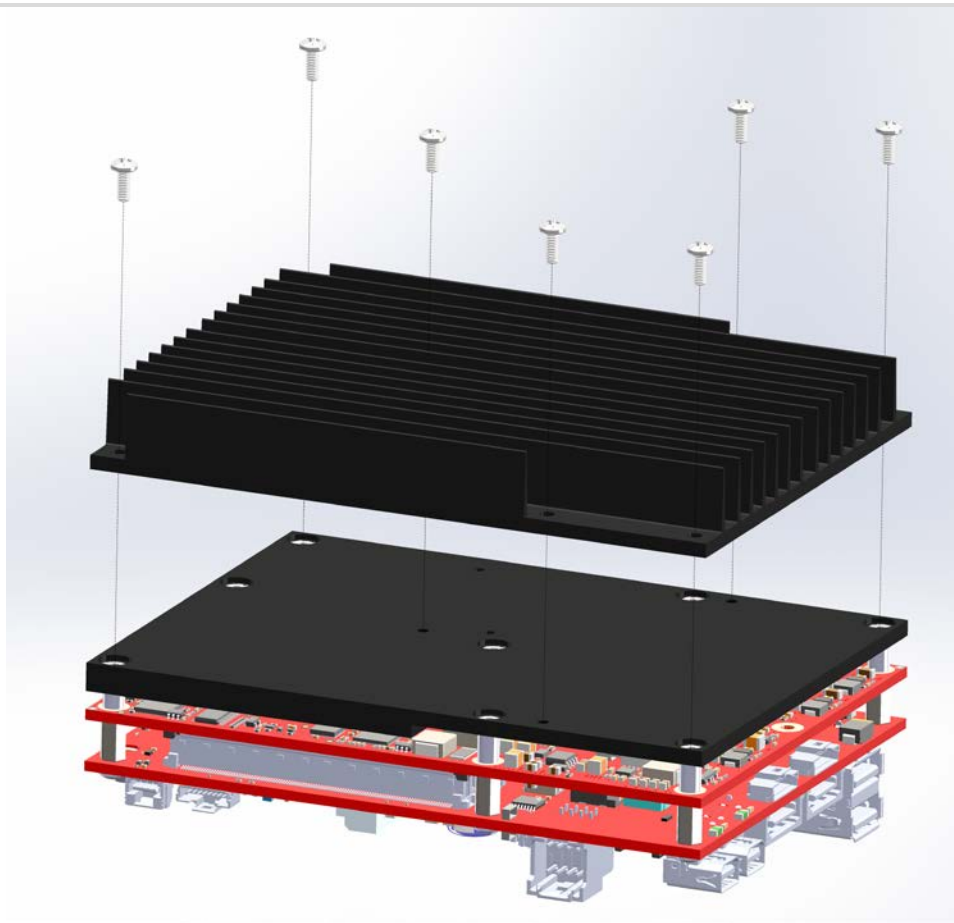
Figure 36. Installing the Passive Heat Sink
