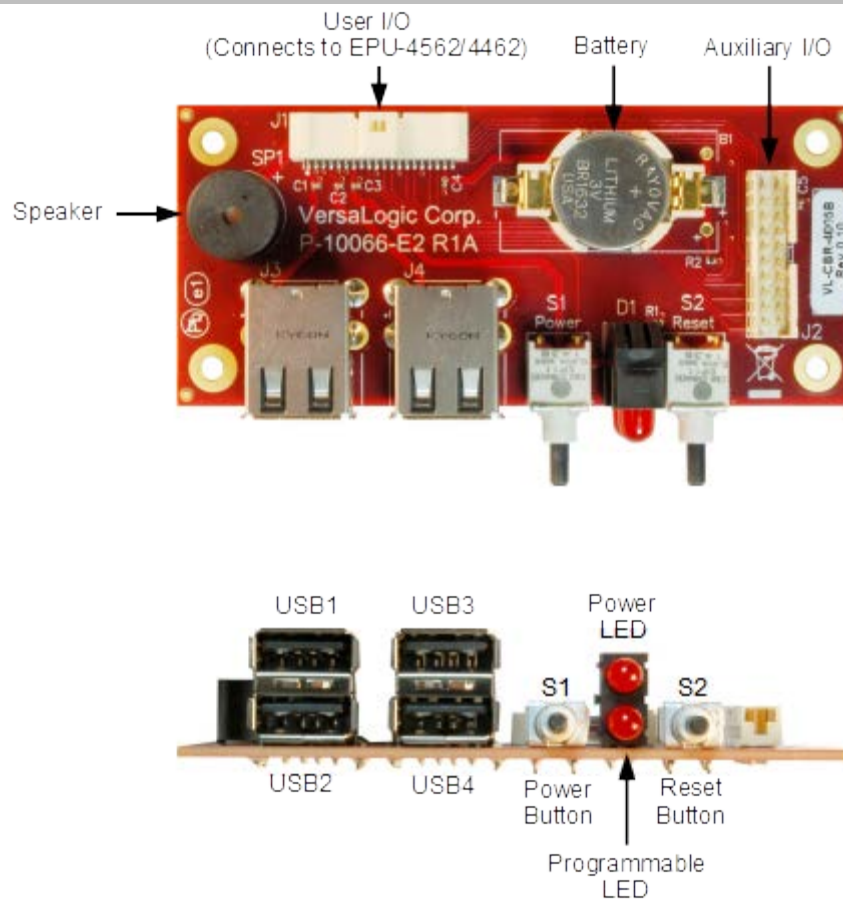
Figure 25. VL-CBR-4005B Connectors, Switches, and LEDs
