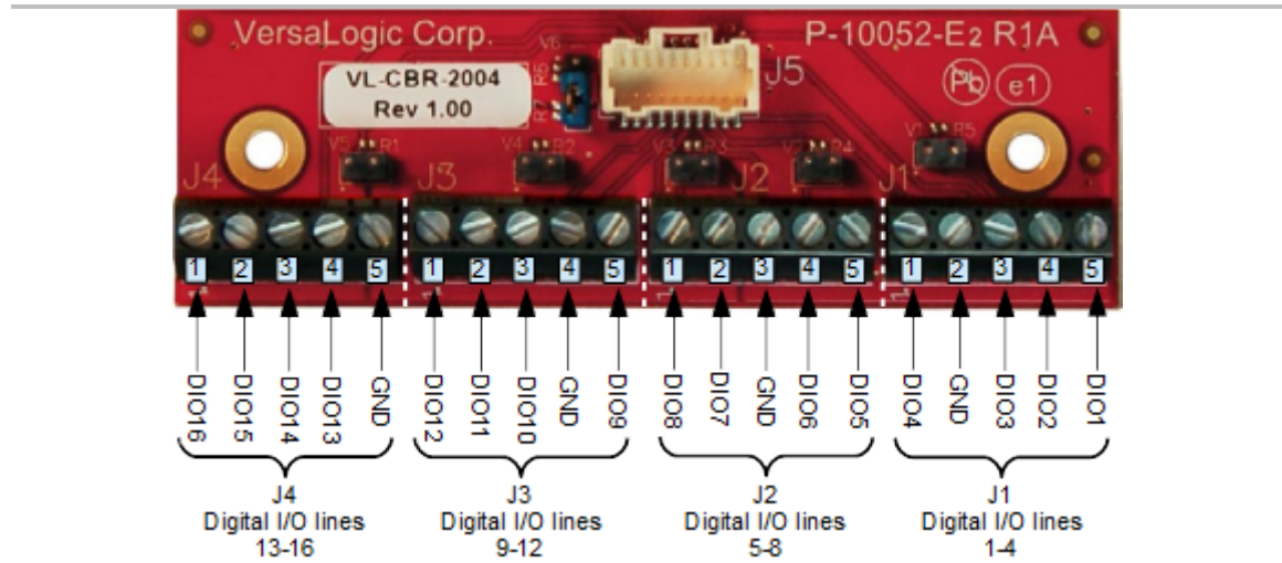
Figure 32. Digital I/O and Ground Terminal Block Pinouts
