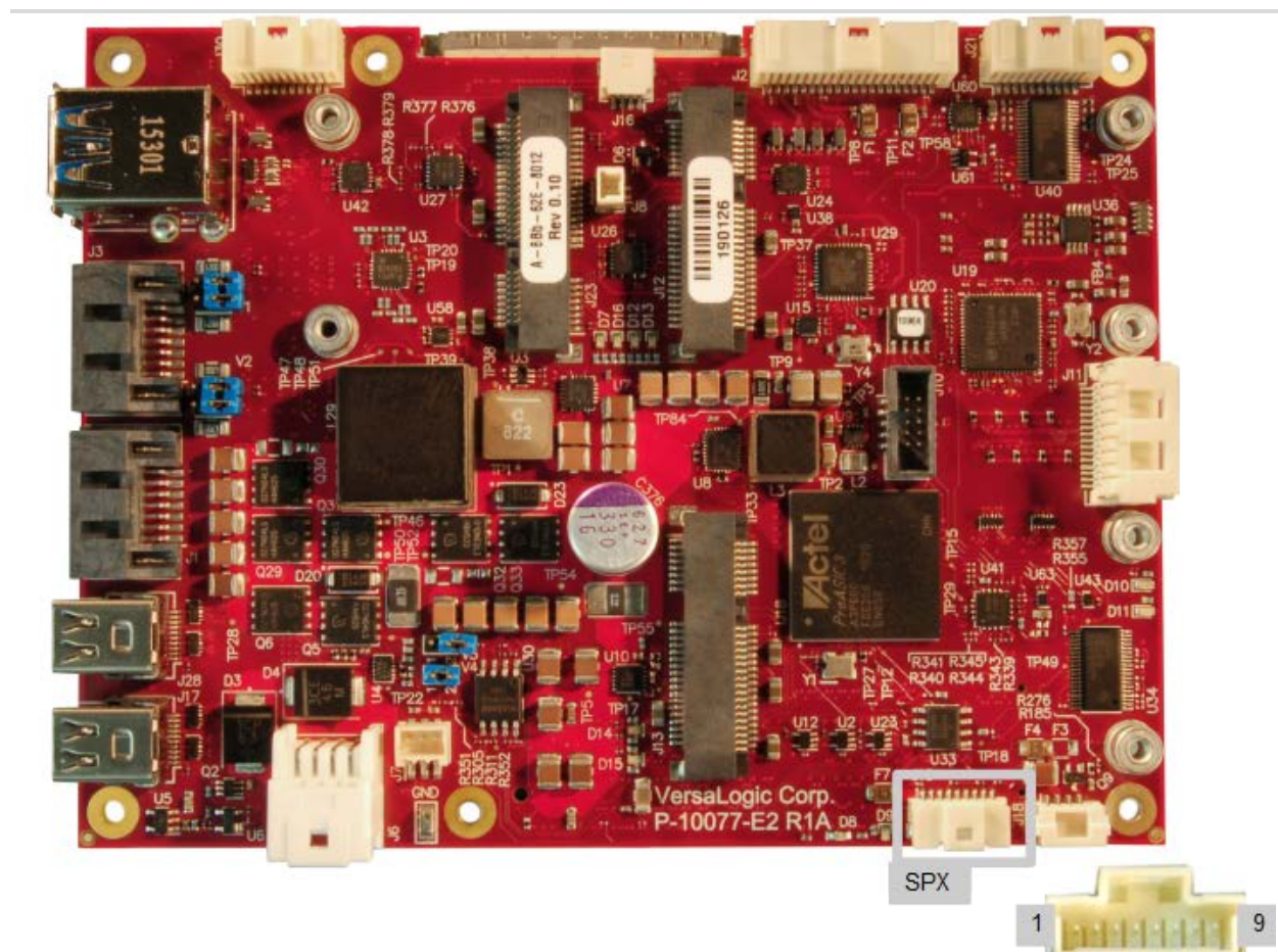
Figure 18. SPX Connector Location and Pin Configuration
