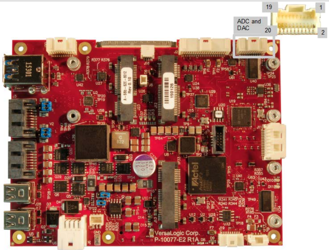
Figure 17. Location and Pin Orientation of the Analog-to-Digital Input Connector
