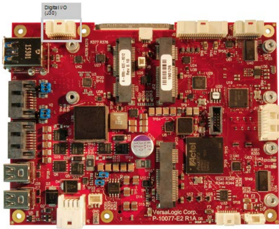
Figure 31: Digital I/O Connector (J30)
