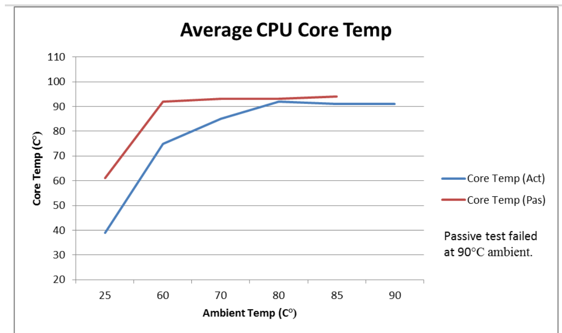
Figure 34. EPU-4562-ECP Quad Core Temperature Relative to Ambient Temperature
