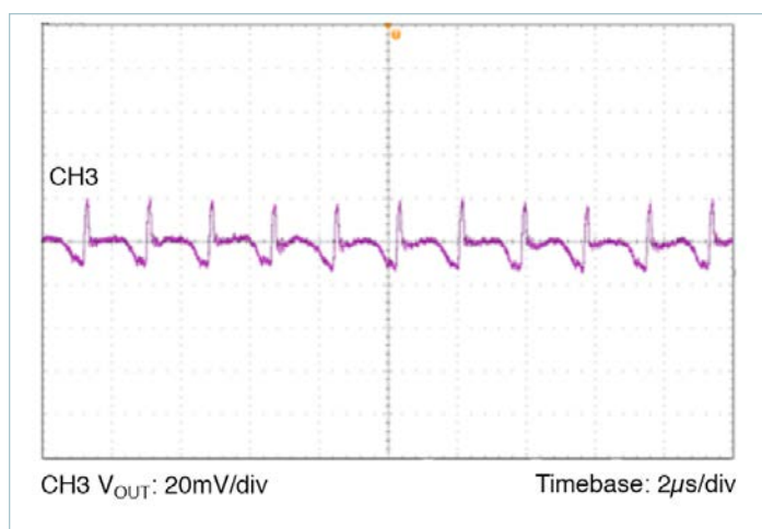
Figure 12 — Output Ripple 24V IN , 1.8V OUT at 7.5A; C_{OUT} = 8 \times 100\mu F Ceramic
