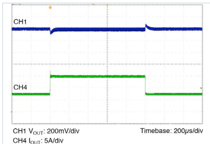
Figure 16 — Transient Response 7.5A to 15A, at 5A/µs; 24V IN to 2.5V OUT , C_{OUT} = 8 \times 100\mu F Ceramic
