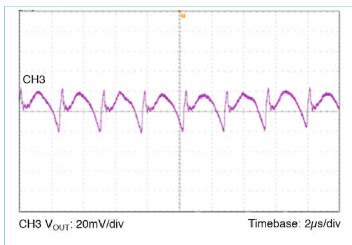
Figure 11 — Output Ripple 24V IN , 1.8V OUT at 15A; C_{OUT} = 8 \times 100\mu F Ceramic
