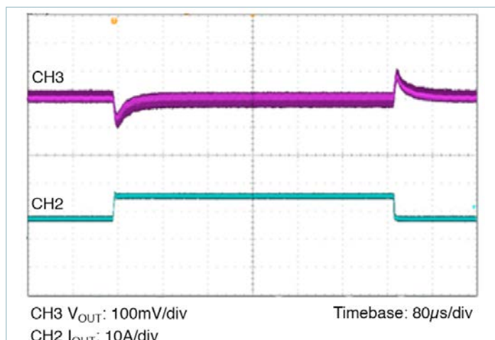
Figure 10 — Transient Response 7A to 15A, at 5A/μs; 24V IN to 1.8V OUT , C_{OUT} = 8 \times 100\mu F Ceramic
