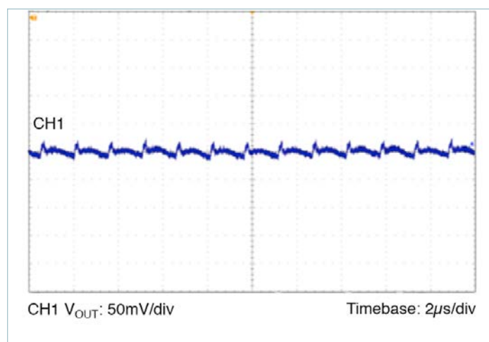
Figure 24 — Output Ripple 24V IN , 3.3V OUT at 7.5A C_{OUT} = 8 \times 100\mu F Ceramic
