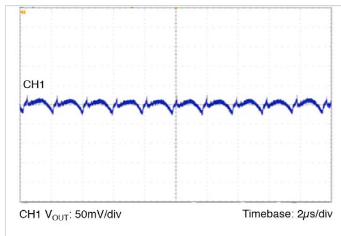
Figure 23 — Output Ripple 24V IN , 3.3V OUT at 15A C_{OUT} = 8 \times 100\mu F Ceramic
