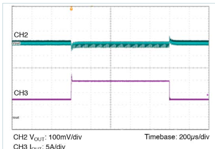
Figure 4 — Transient Response 7.5A to 15A, at 5A/ \mu s ; 24V IN to 1.0V OUT , C_{OUT} = 8 \times 100\mu F Ceramic
