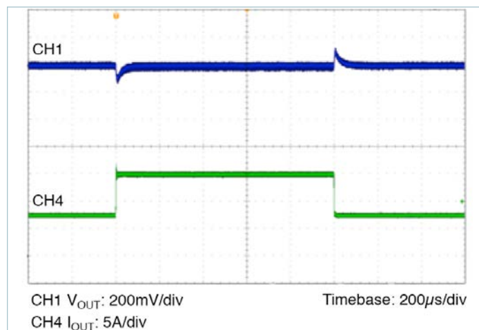
Figure 22 — Transient Response 7.5A to 15A, at 5A/μs 24V IN to 3.3V OUT , C_{OUT} = 8 \times 100\mu F Ceramic
