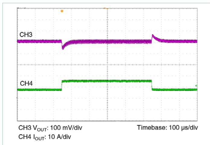
Figure 16 — 12 V_{IN} to 2.5 V_{OUT} , C_{OUT} = 8 X 100 \mu F Ceramic V_{OUT} (Ch2) = 100 mV/div, I_{IN} (Ch1) = 10 A/div, 100 \mu s/div
