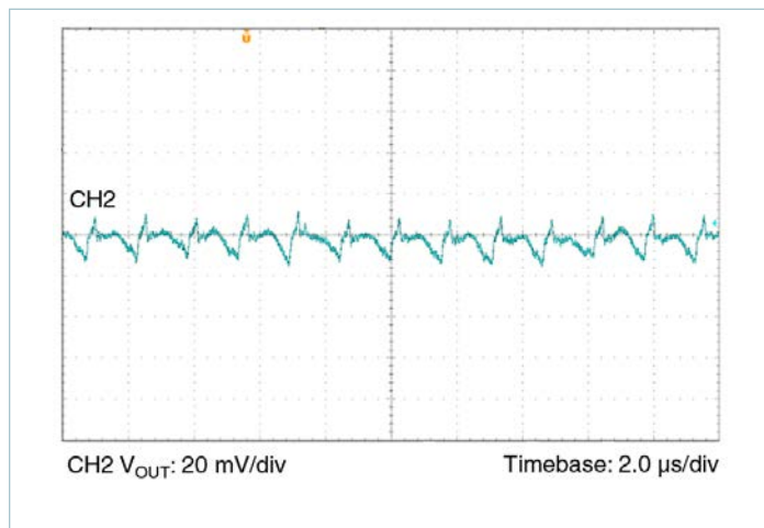
Figure 18 — Output Ripple 12 V_{IN} 2.5 V_{OUT} at 7.0 A; C_{OUT} = 8 x 100 \mu F
