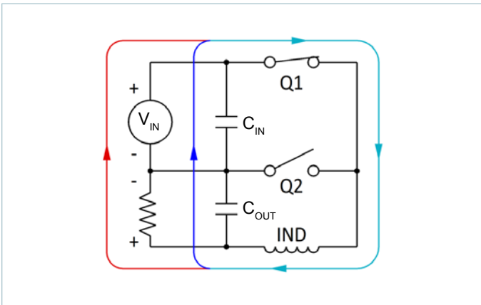
Figure 42 — Current flow: Q1 closed
