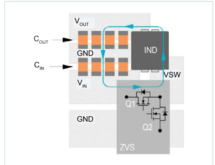
Figure 44 — Recommended component placement and metal routing
