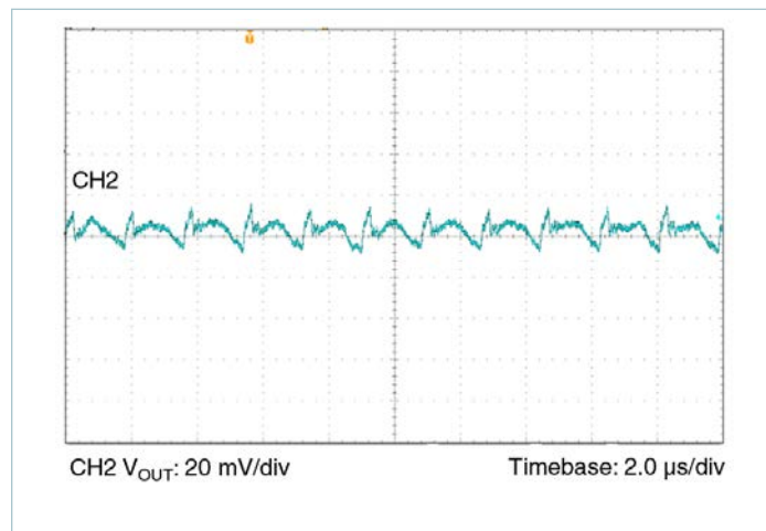
Figure 12 — Output Ripple 12 V IN 1.8 V OUT at 7.0 A; C_{OUT} = 8 \times 100 \mu F
