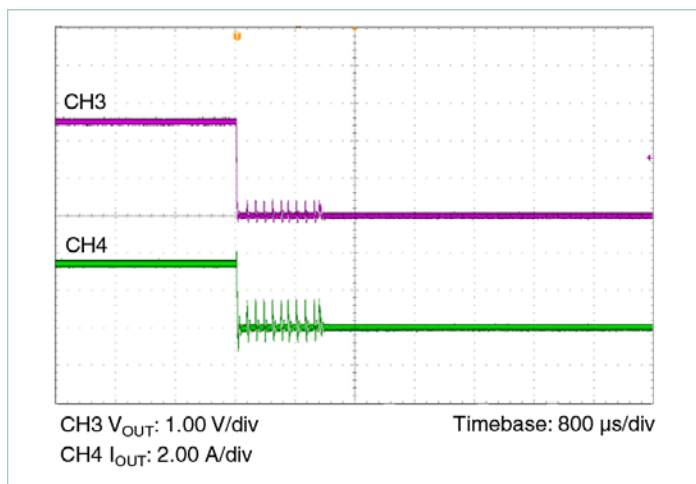
Figure 14 — V_{OUT} (Ch3) = 1V/div, I_{IN} (Ch4) = 2 A/div, 800 \mu s/div
