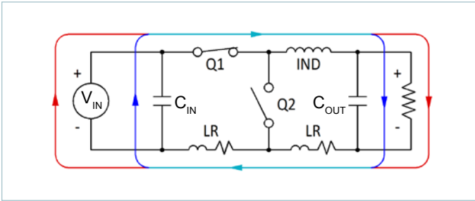
Figure 41 — Typical Buck Regulator
