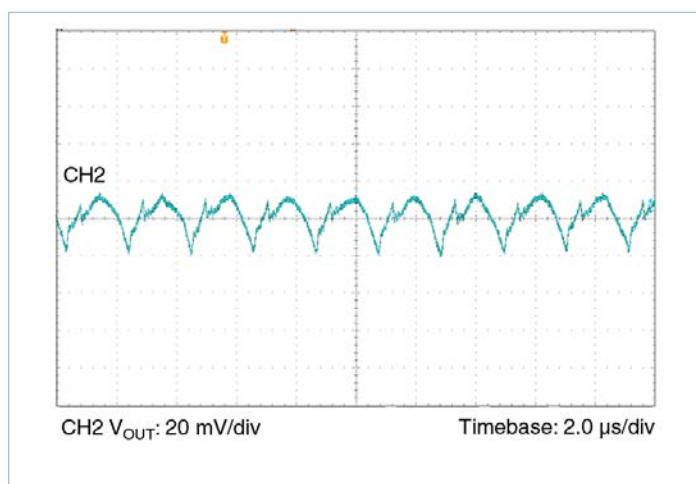
Figure 17 — Output Ripple 12 V_{IN} 2.5 V_{OUT} at 15 A; C_{OUT} = 8 x 100 \mu F
