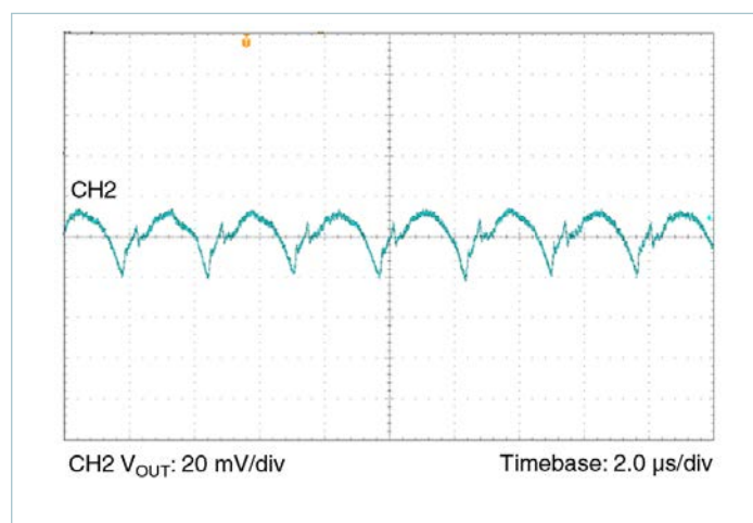
Figure 11 — Output Ripple 12 V IN 1.8 V OUT at 15 A; C_{OUT} = 8 \times 100 \mu F
