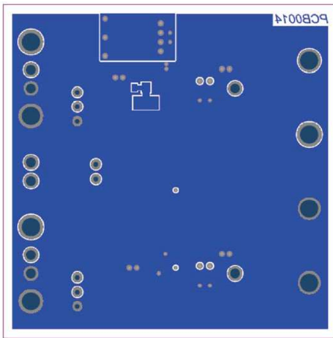
Figure 7d – PI2001-EVAL1 layout Bottom layer. Scale 2.0:1
