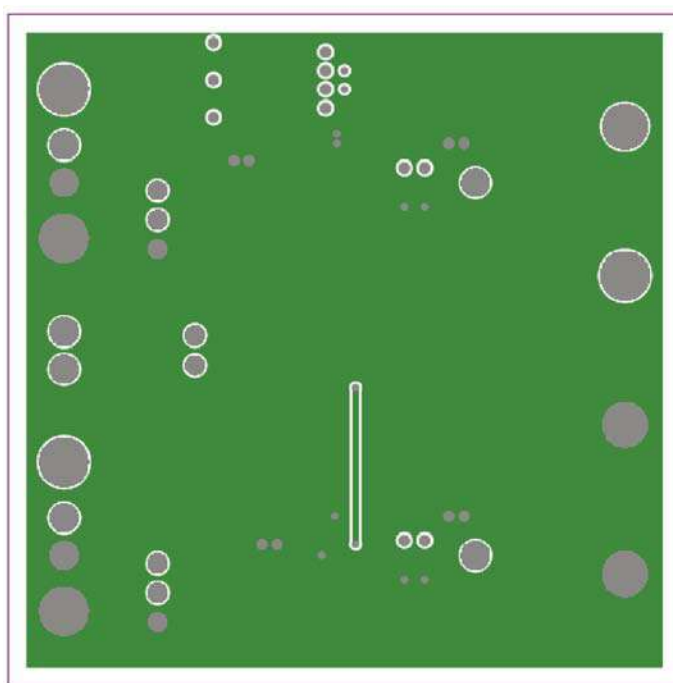
Figure 7b – PI2001-EVAL1 layout mid layer 2. Scale 2.0:1
