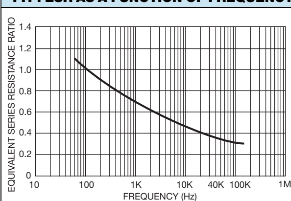
TYP. ESR AS A FUNCTION OF FREQUENCY
