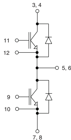
Fig. 25 - Electrical diagram
