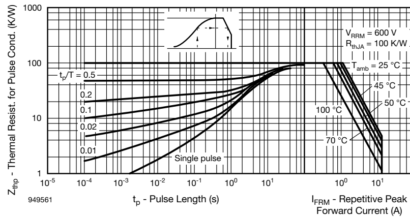
Fig. 7 - Thermal Response
