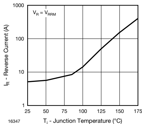
Fig. 4 - Reverse Current vs. Junction Temperature ( ^{\circ}\text{C} )
