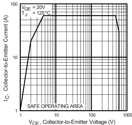
Fig. 12 - Turn-Off SOA
