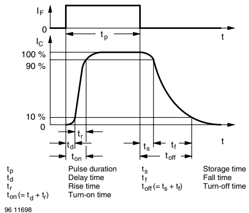
Fig. 5 - Switching Times
