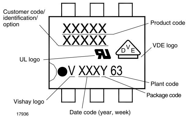
Fig. 18 - Marking Example
