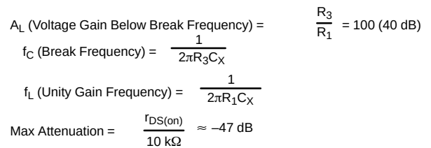
FIGURE 7. Active Low Pass Filter with Digitally Selected Break Frequency
