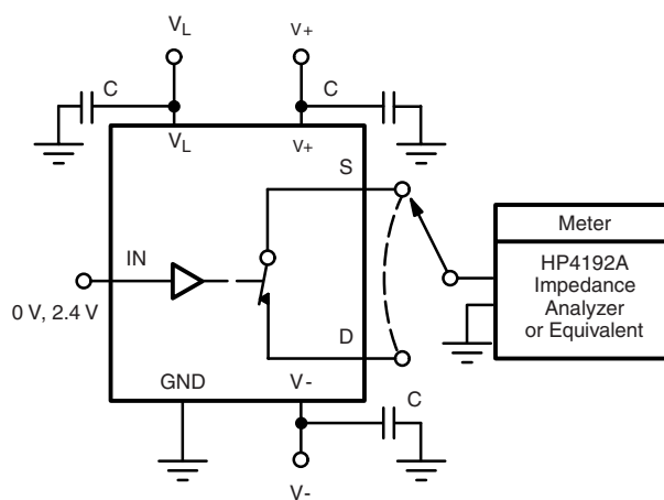
Figure 7. Source/Drain Capacitances
