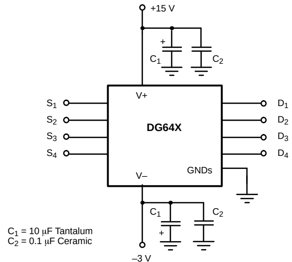
FIGURE 7. Supply Decoupling
