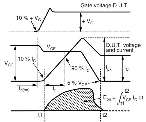
Fig. 17c - Test Waveforms for Circuit of Fig. 18a, Defining E_{on} , t_{d(on)} , t_r
