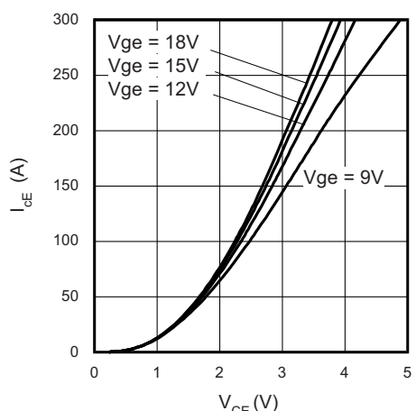
Fig. 2 - Typical IGBT Output Characteristics T_J = 125^{\circ}\text{C} , t_p = 500\text{ }\mu\text{s}
