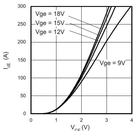
Fig. 1 - Typical IGBT Output Characteristics T_J = 25^{\circ}\text{C} , t_p = 500\text{ }\mu\text{s}
