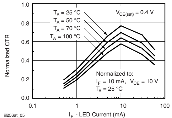
Fig. 5 - Normalized Saturated CTR
