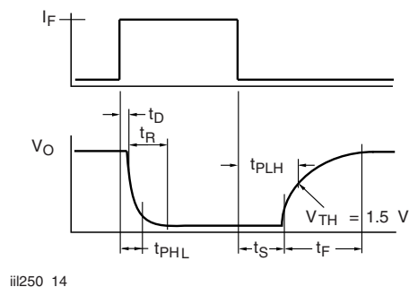
Fig. 14 - Switching Timing
