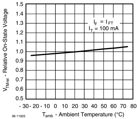
Fig. 9 - Relativ On-State Current vs. Ambient Temperature
