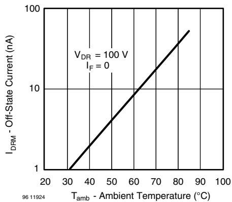
Fig. 10 - Off-State Current vs. Ambient Temperature
