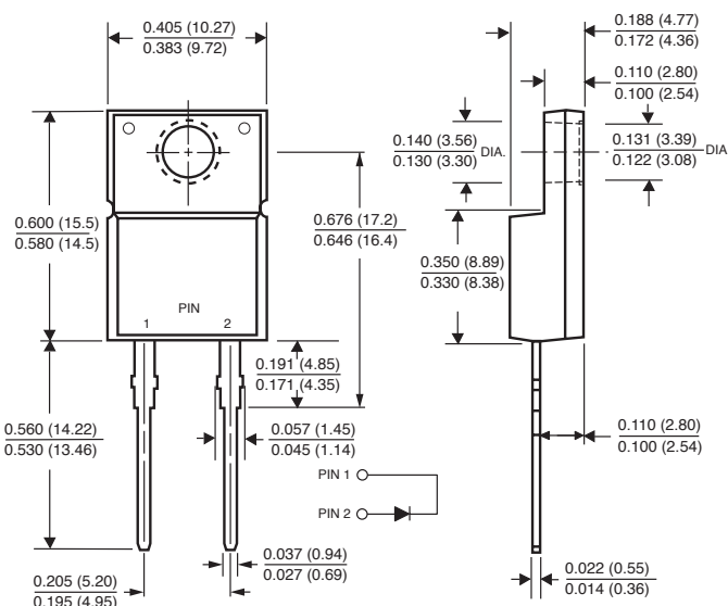
ITO-220AC (MBRF16xx)
