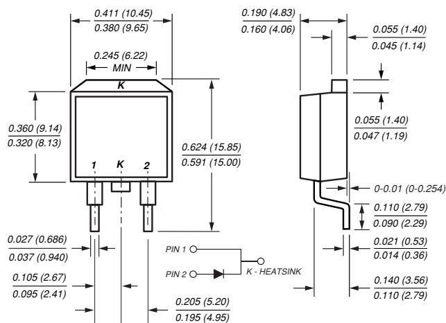
TO-263AB (MBRB16xx)
