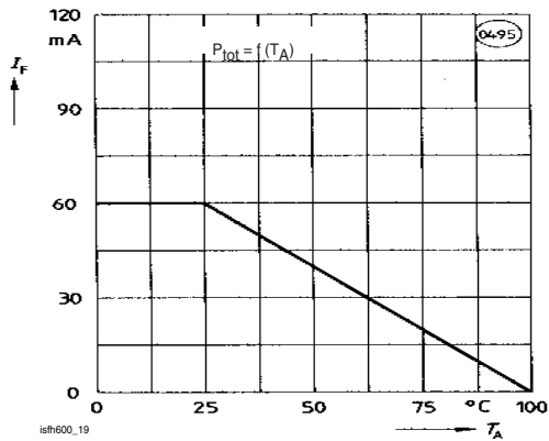
Fig. 19 Permissible Forward Current Diode
