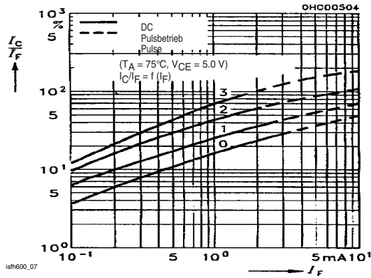
Fig. 7 Current Transfer Ratio vs. Diode Current
