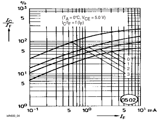
Fig. 4 Current Transfer Ratio vs. Diode Current
