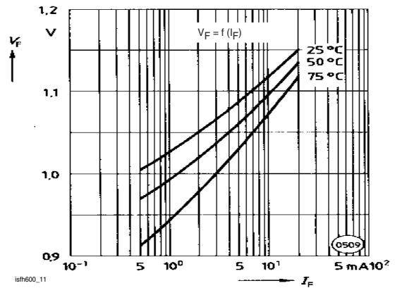
Fig. 11 Forward Voltage
