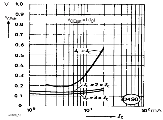
Fig. 16 Saturation Voltage vs. Collector Current and Modulation Depth SFH600-3
