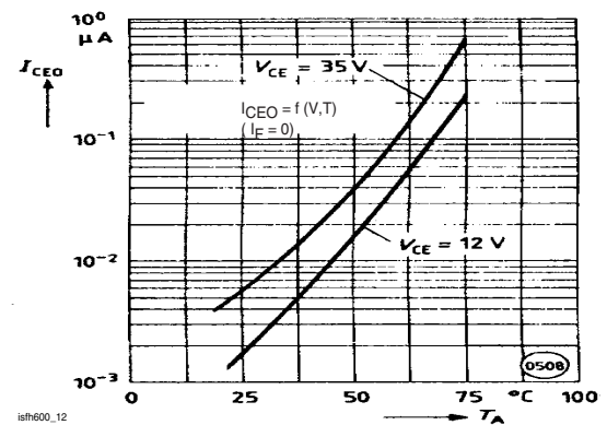
Fig. 12 Collector-Emitter Off-state Current
