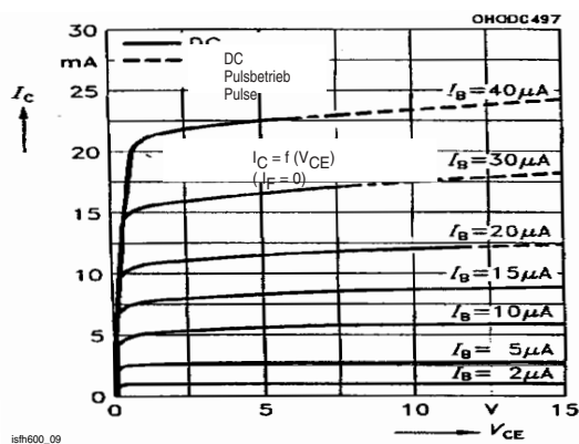
Fig. 9 Transistor Characteristics SFH600-2, -3
