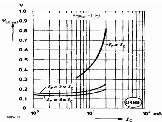
Fig. 15 Saturation Voltage vs. Collector Current and Modulation Depth SFH600-2
