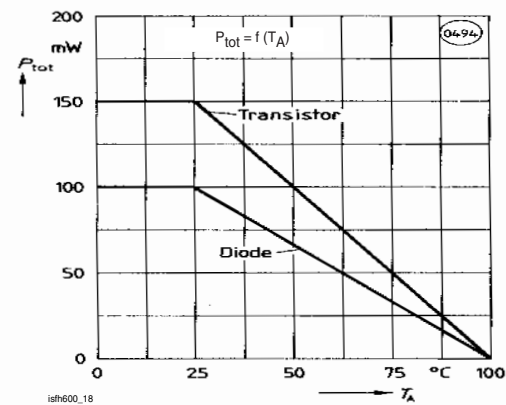
Fig. 18 Permissible Power Dissipation for Transistor and Diode
