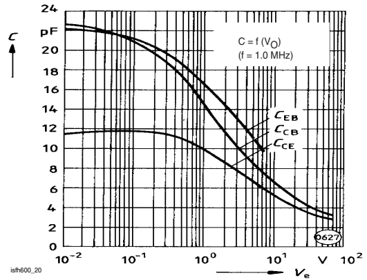
Fig. 20 Transistor Capacitance
