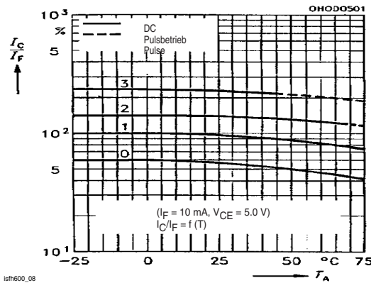
Fig. 8 Current Transfer Ratio (CTR) vs. Temperature
