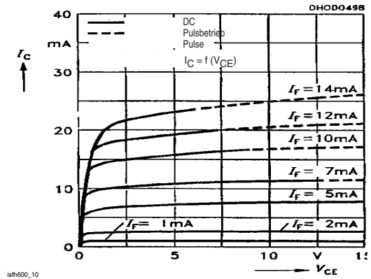
Fig. 10 Output Characteristics SFH600-2, -3
