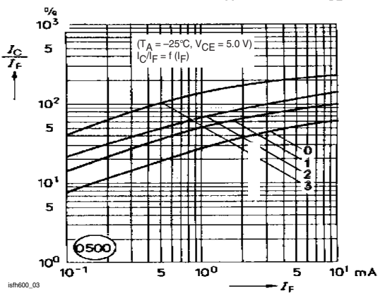
Fig. 3 Current Transfer Ratio vs. Diode Current
