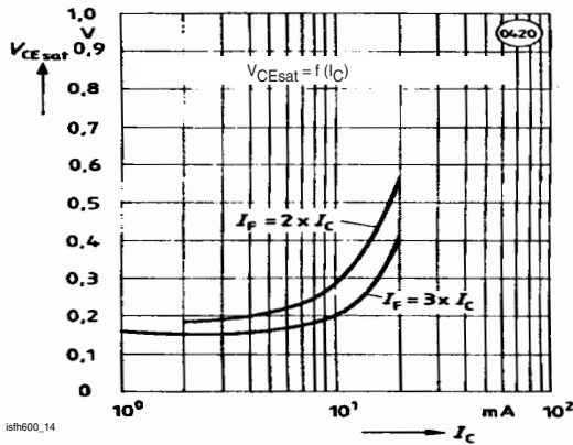
Fig. 14 Saturation Voltage vs. Collector Current and Modulation Depth SFH600-1
