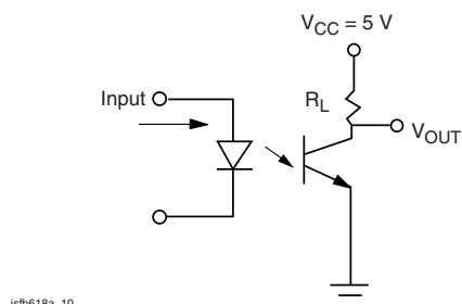
Fig. 2 - Test Circuit
