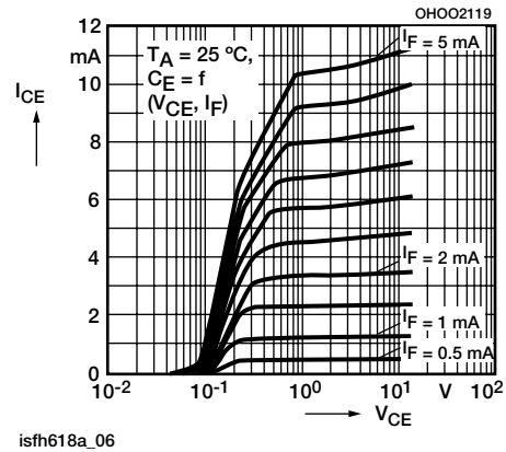
Fig. 9 - Output Characteristics
