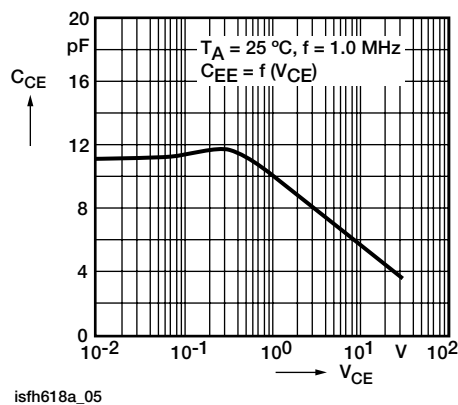
Fig. 8 - Transistor Capacitance
