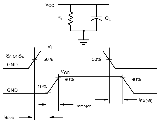
FIGURE 2. t_{\text{ramp}(on)}
