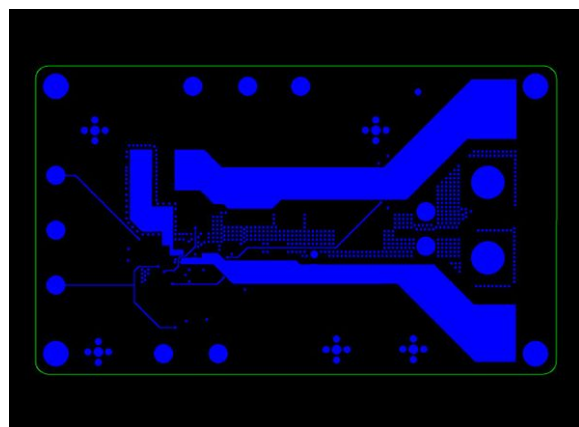
Figure 16. Mid Layer2
