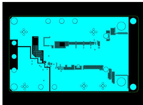
Figure 15. Mid Layer1
