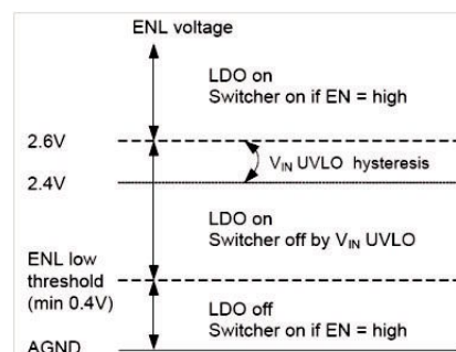
Figure 11 - ENL Thresholds
