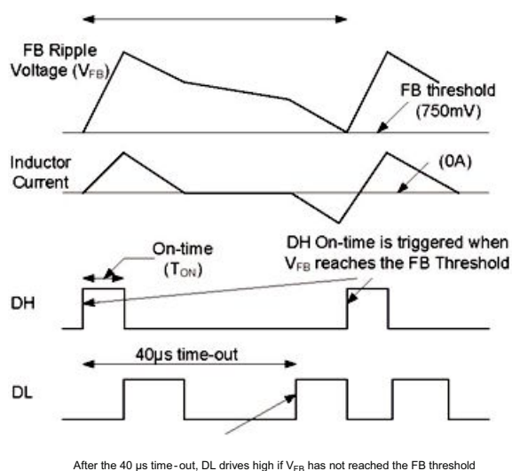
Figure 5 - Ultrasonic Power-Save Operation
