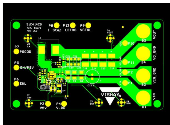
Figure 14. Top Layer
