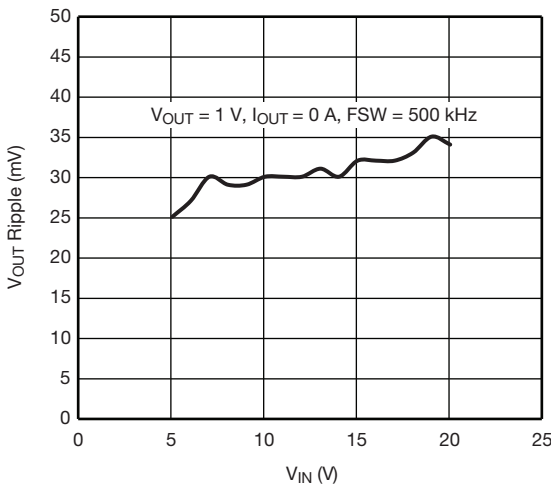
V_{OUT} Ripple vs. V_{IN} ( I_{OUT} = 0 A in Continuous Conduction Mode)
