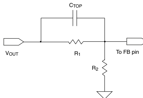
Figure 11 - Capacitor Coupling to FB Pin
