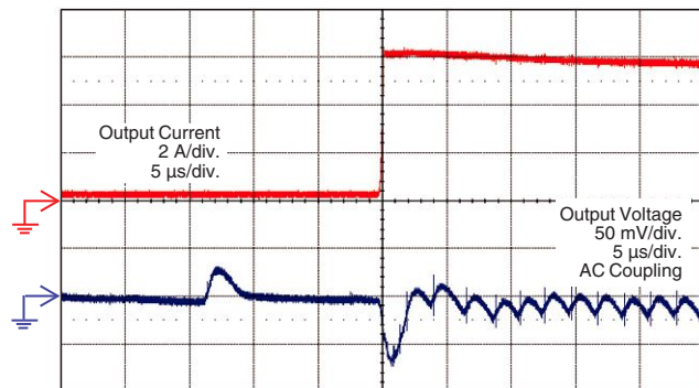
Transient Response in Power Save Mode (0.2 A - 6 A) (V_{IN} = 12\text{ V}, V_{OUT} = 1\text{ V}, F_{SW} = 500\text{ kHz at 6A})
