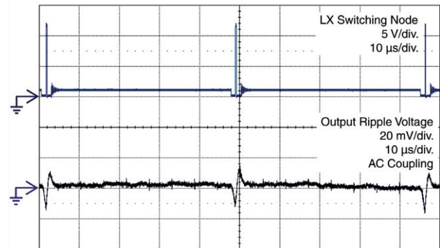
V_{OUT} Ripple in Power Save Mode (No Load) (V_{IN} = 12\text{ V}, V_{OUT} = 1\text{ V})
