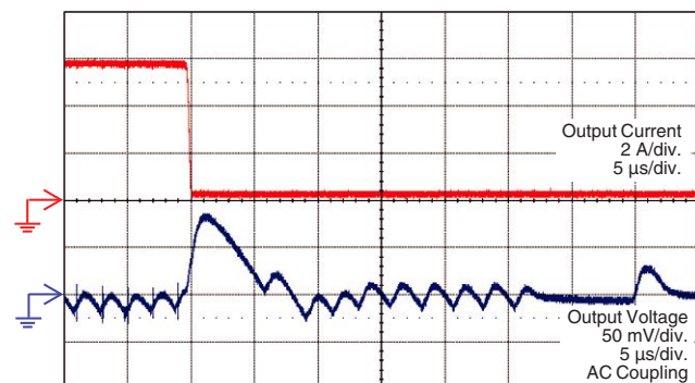
Transient Response in Power Save Mode (6 A - 0.2 A) (V_{IN} = 12\text{ V}, V_{OUT} = 1\text{ V}, F_{SW} = 500\text{ kHz at 6A})
