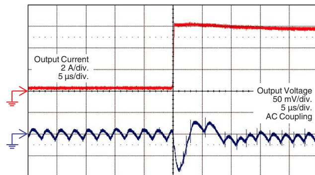
Transient Response in Continuous Conduction Mode (0.2 A - 6 A) (V_{IN} = 12\text{ V}, V_{OUT} = 1\text{ V}, F_{SW} = 500\text{ kHz})
