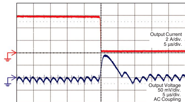
Transient Response in Continuous Conduction Mode (6 A - 0.2 A) (V_{IN} = 12\text{ V}, V_{OUT} = 1\text{ V}, F_{SW} = 500\text{ kHz})
