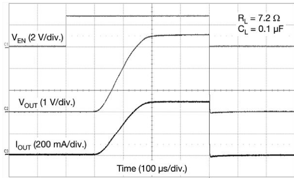
Figure 21 - Switching ( V_{IN} = 3.6\text{ V} )
