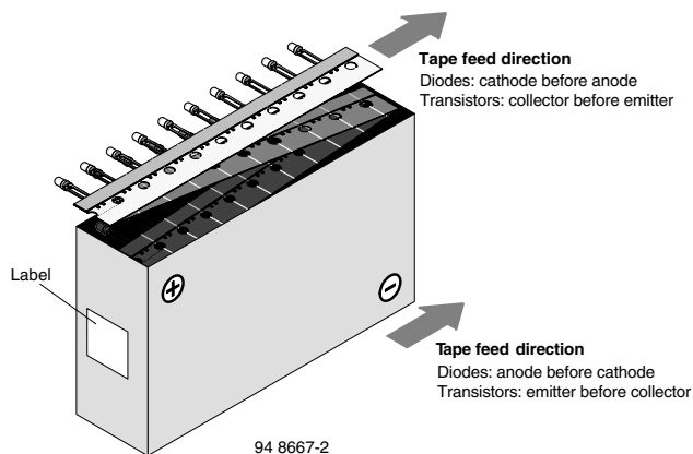
Fig. 20 - Tape Direction
