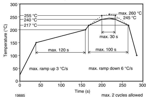
Fig. 12 - Vishay Lead (Pb)-free Reflow Soldering Profile (acc. to J-STD-020C)
