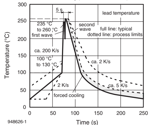
Figure 13. Double Wave Soldering of Opto Devices (all Packages)
