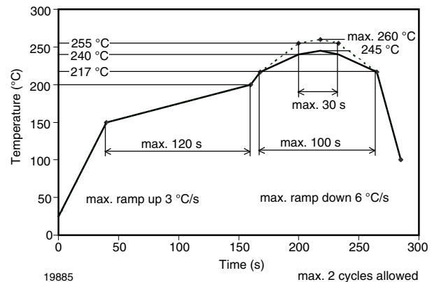
Figure 12. Vishay Lead (Pb)-free Reflow Soldering Profile (acc. to J-STD-020)
