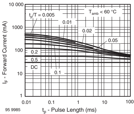
Figure 2. Permissible Pulse Forward Current vs. Pulse Length
