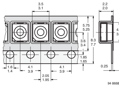
Figure 10. Tape Dimensions in mm for PLCC-2
