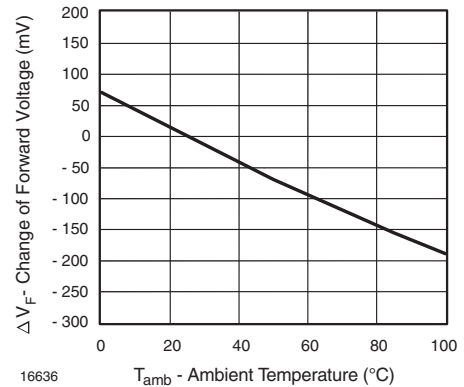
Figure 6. Change of Forward Voltage vs. Ambient Temperature
