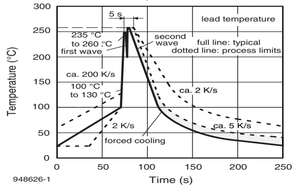
Fig. 10 - Double Wave Soldering of Opto Devices (all Packages)
