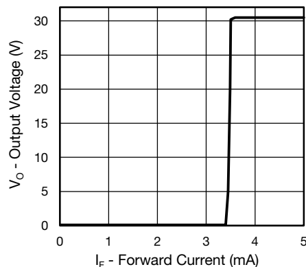
Fig. 15 - Output Voltage vs. Forward Current
