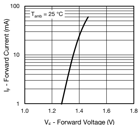
Fig. 21 - Forward Current vs. Forward Voltage
