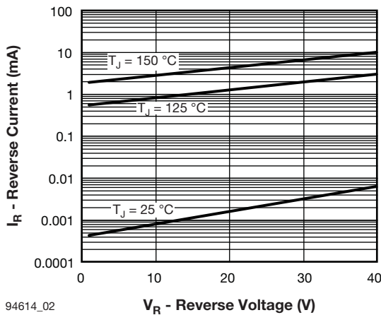
94614_02 V R - Reverse Voltage (V) Fig. 2 - Typical Values of Reverse Current vs. Reverse Voltage
