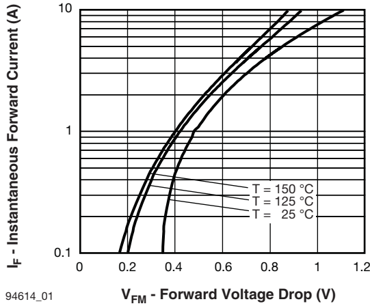
94614_01 V FM - Forward Voltage Drop (V) Fig. 1 - Maximum Forward Voltage Drop Characteristics
