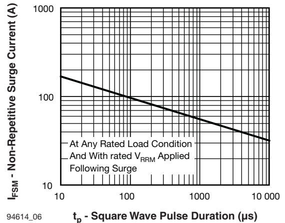
94614_06 t p - Square Wave Pulse Duration (μs) Fig. 6 - Typical Non-Repetitive Surge Current
