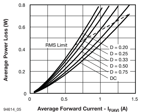
94614_05 Average Forward Current - I F(AV) (A) Fig. 5 - Forward Power Loss Characteristics
