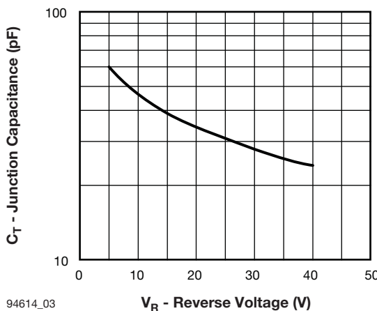
94614_03 V R - Reverse Voltage (V) Fig. 3 - Typical Junction Capacitance vs. Reverse Voltage
