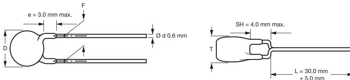
Capacitors with 10 mm lead spacing
