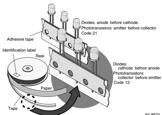
Figure 40. LED in Tape
