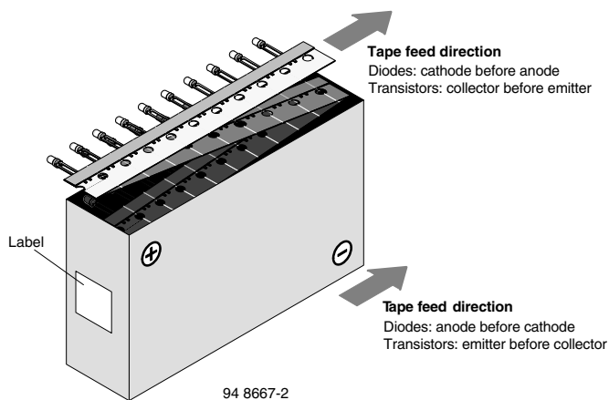
Fig. 16 - Tape Direction
