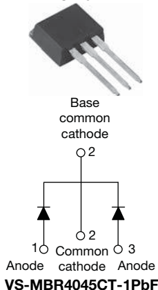
TO-262AA
