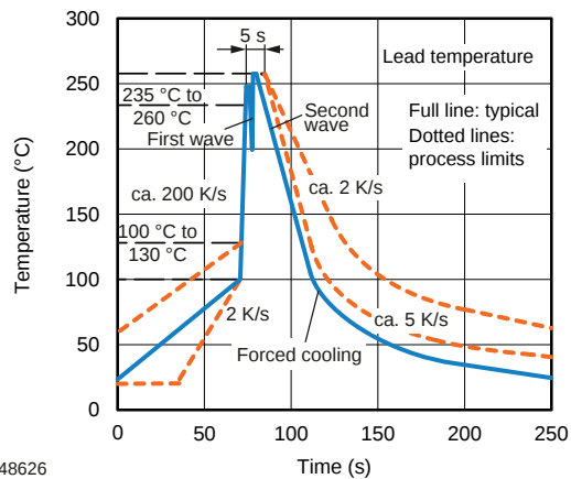
Fig. 6 - Wave Soldering Double Wave Profile According to J-STD-020 for DIP Devices
