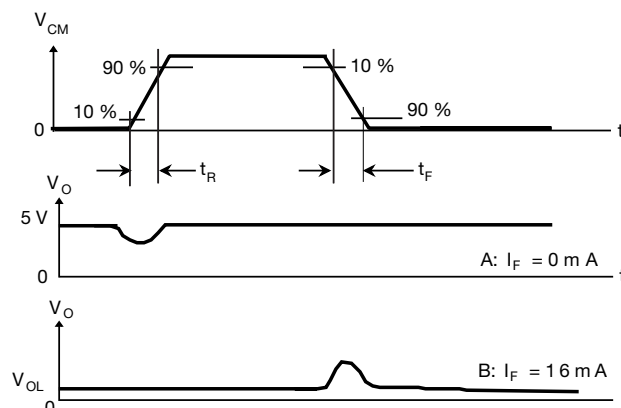
Fig. 6 - Measurement Waveform of CMR
