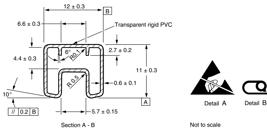
Fig. 15 - Tube Shipping Medium
