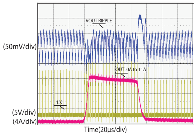
Transient Response - FCM ( V_{DD} = 5\text{ V} , V_{IN} = 12\text{ V} , V_{OUT} = 1.5\text{ V} , I_{OUT} = 0\text{ A} to 11\text{ A} , SiC401B, dl/dt = 1\text{ A}/\mu\text{s} )
