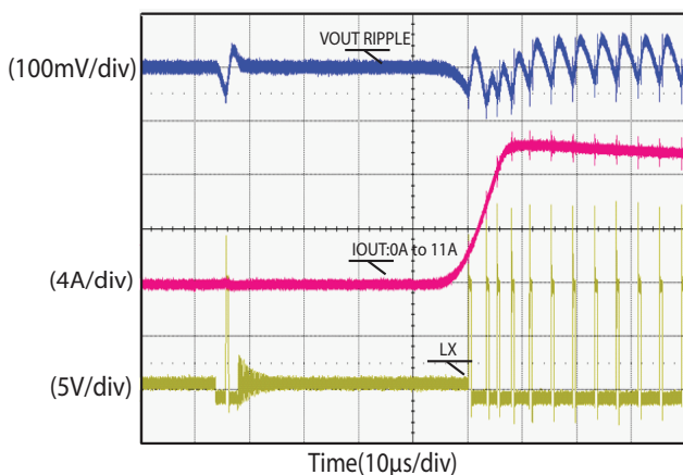
Transient Response - P-Save Load Rising ( V_{DD} = 5\text{ V} , V_{IN} = 12\text{ V} , V_{OUT} = 1.5\text{ V} , I_{OUT} = 0\text{ A} to 11\text{ A} , SiC401A, dl/dt = 1\text{ A}/\mu\text{s} )
