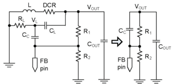
Fig. 16 - FB Voltage by Output Voltage
