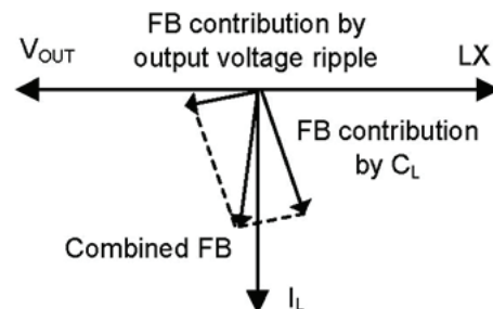
Fig. 17 - FB Voltage in Phasor Diagram
