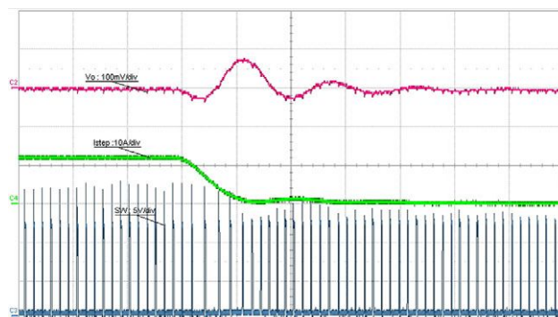
Fig. 27 - Load Release, 12 A to 0.1 A, 1 A/ \mu s, t = 10 \mu s/div. Forced Continuous Conduction Mode
