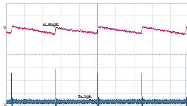
Fig. 28 - Output Ripple, 0.01 A, t = 1 \mu s/div. DCM Mode
