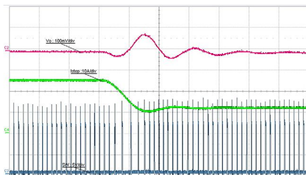
Fig. 22 - Load Release, 25 A to 12 A, 1 A/μs, t = 10 \text{ μs/div} .
