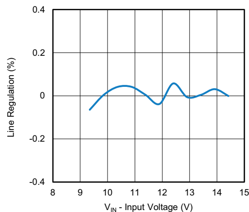
Fig. 15 - Line Regulation
