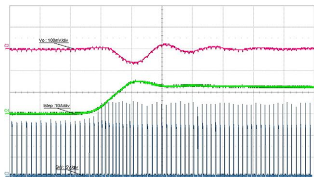
Fig. 24 - Load Step, 0.1 A to 12 A, 1 A/ \mu s, t = 10 \mu s/div. Forced Continuous Conduction Mode
