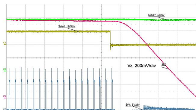
Fig. 18 - Overcurrent Protection Behavior, t = 5 \text{ μs/div} .
