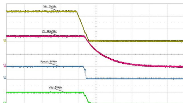
Fig. 16 - Shut Down With V_{IN} , t = 100\text{ ms/div} .
