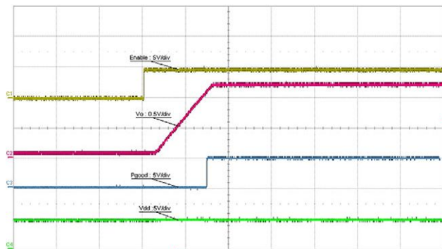
Fig. 17 - Startup With EN, t = 5 \text{ ms/div} .
