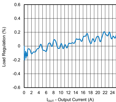
Fig. 12 - Load Regulation
