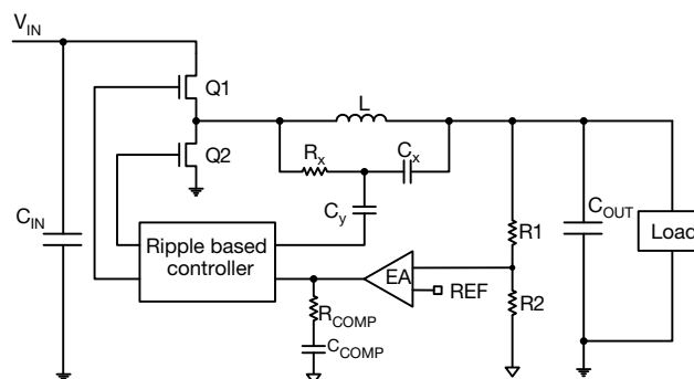
Fig. 5 - VM-COT Block Diagram
