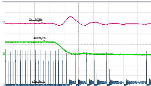
Fig. 26 - Load Release, 12 A to 0.1 A, 1 A/ \mu s, t = 10 \mu s/div. Skip Mode Enabled
