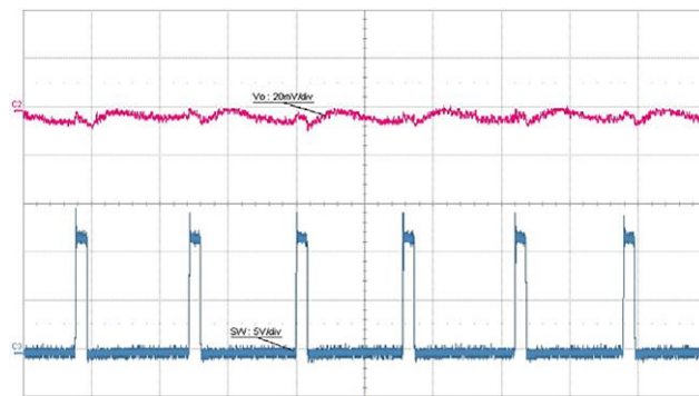
Fig. 25 - Output Ripple, 0.01 A, t = 1 \mu s/div. Forced Continuous Conduction Mode
