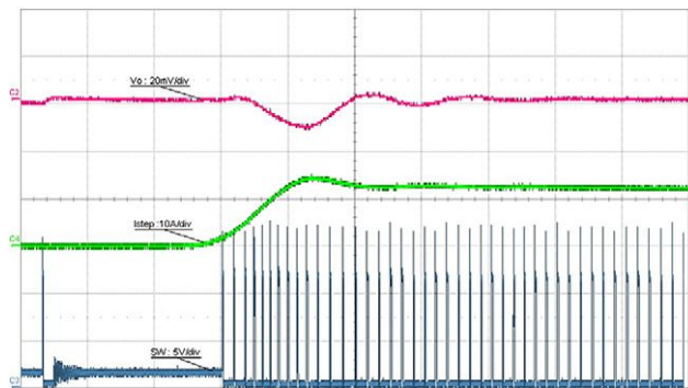
Fig. 23 - Load Step, 0.1 A to 12 A, 1 A/ \mu s, t = 10 \mu s/div. Skip Mode Enabled
