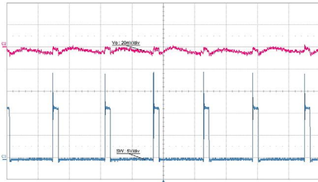
Fig. 29 - Output Ripple, 12 A, t = 1 \mu\text{s}/\text{div} .
