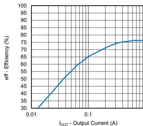
Fig. 14 - Efficiency vs. Output Current - Light Load
