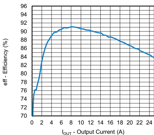
Fig. 11 - Efficiency vs. Output Current
