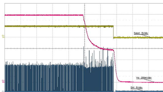
Fig. 21 - Output Undervoltage Protection Behavior, t = 100 \text{ μs/div} .
