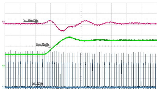
Fig. 19 - Load Step, 12 A to 25 A, 1 A/μs, t = 10 \text{ μs/div} .
