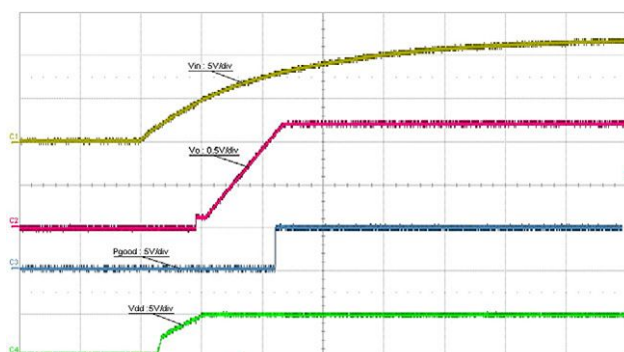
Fig. 13 - Startup With V_{IN} , t = 5\text{ ms/div} .
