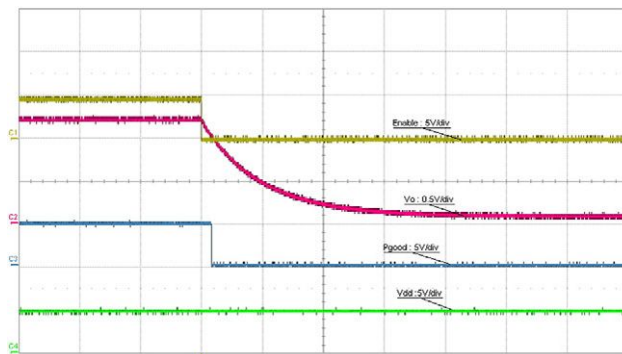
Fig. 20 - Shut Down With EN, t = 100 \text{ ms/div} .
