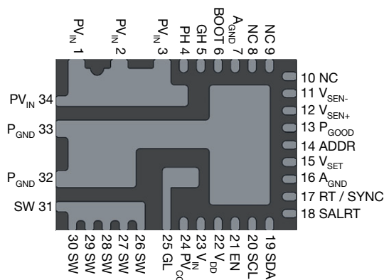
Fig. 4 - Pin Configuration - Bottom View
