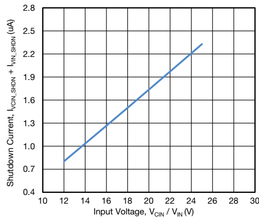
Fig. 16 - Shutdown Current vs. Input Voltage
