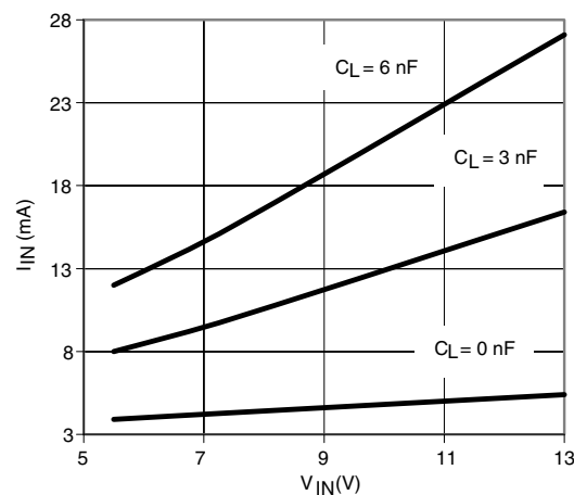
250 kHz Supply Current vs. C_L
