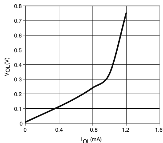
Error Amp V_{OL} vs. I_{OL}
