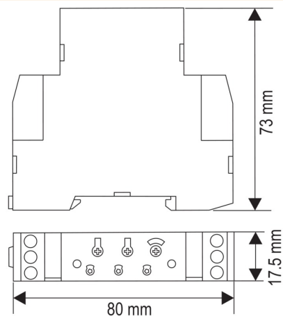
Dimensioned drawing
