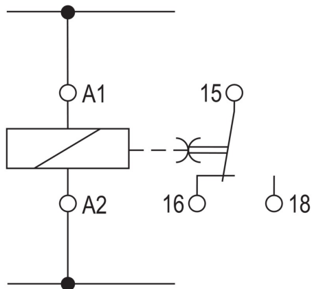
Wiring diagram
