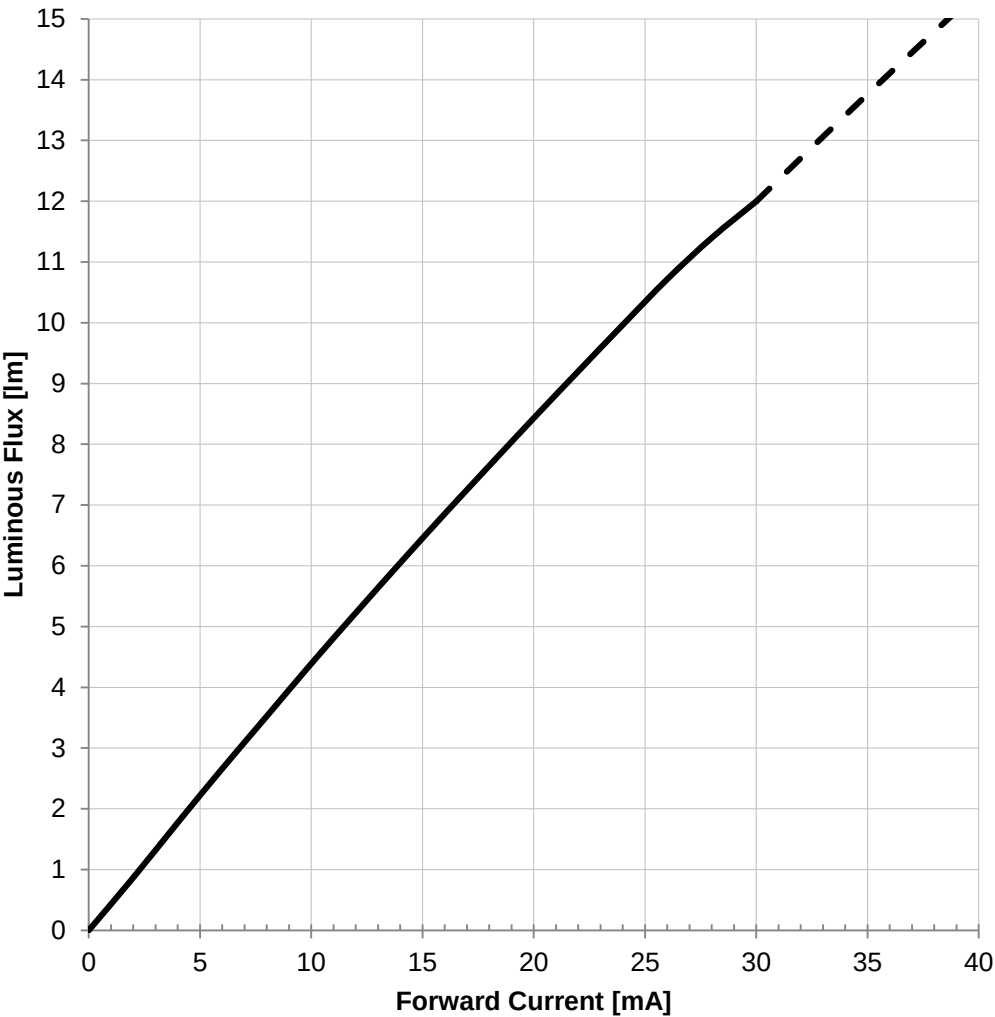
Luminous Flux vs. Forward current:
